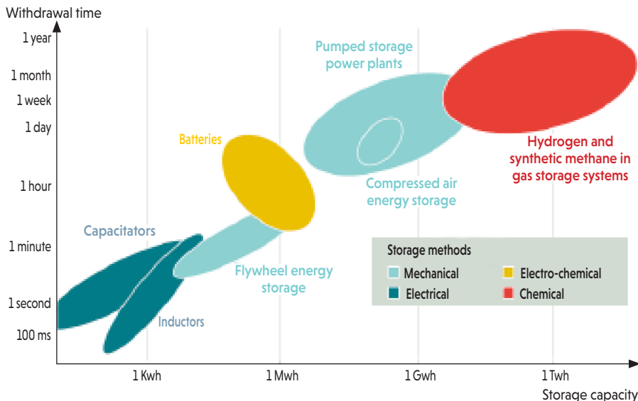
A COMPARISON OF DIFFERENT ENERGY STORAGE TECHNOLOGIES
